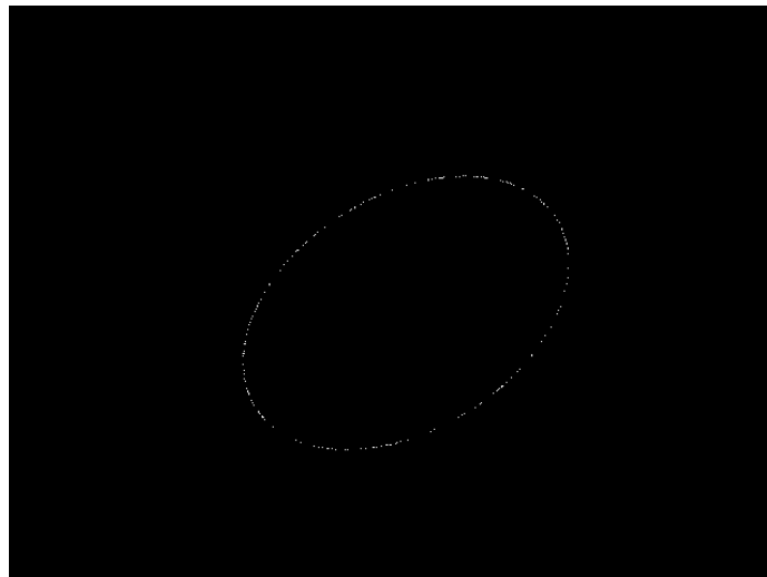
Figure 4.8.2: glm::vec4(glm::circularRand(1.0f), 0, 1);
