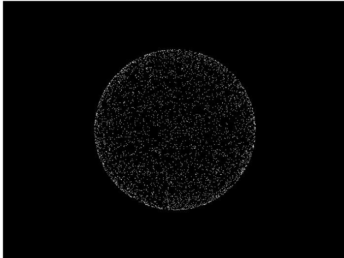
Figure 5.7.3: glm::vec4(glm::sphericalRand(1.0f), 1);
