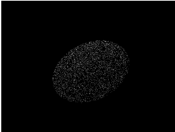
Figure 5.7.4: glm::vec4(glm::diskRand(1.0f), 0, 1);
