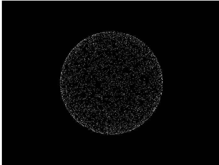
Figure 5.10.3: glm::vec4(glm::sphericalRand(1.0f), 1);
