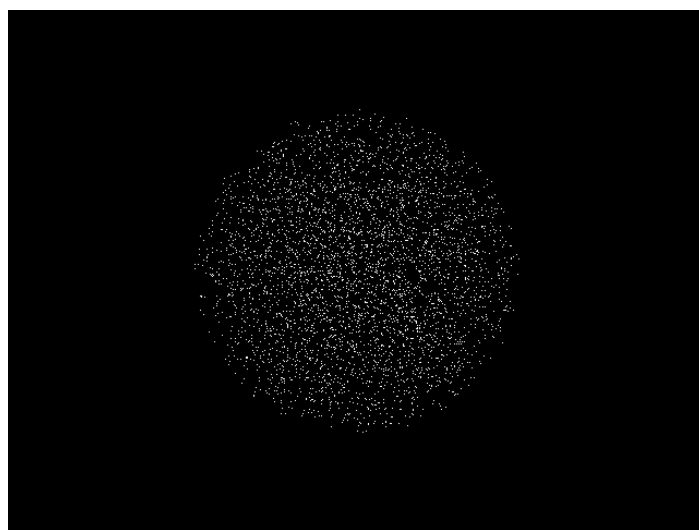
Figure 4.13.5: glm::vec4(glm::ballRand(1.0f), 1);
