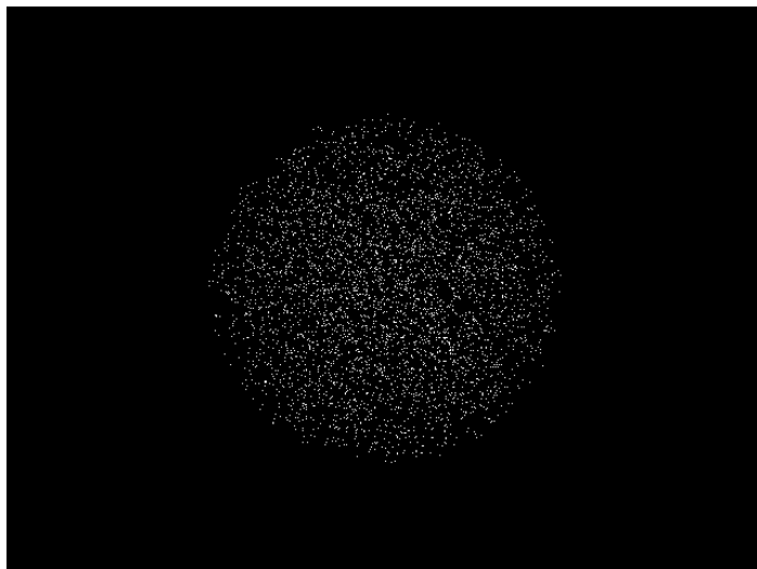
Figure 4.8.5: glm::vec4(glm::ballRand(1.0f), 1);
